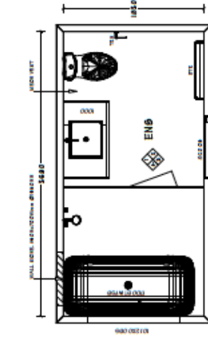
ENS DETAIL PLAN
