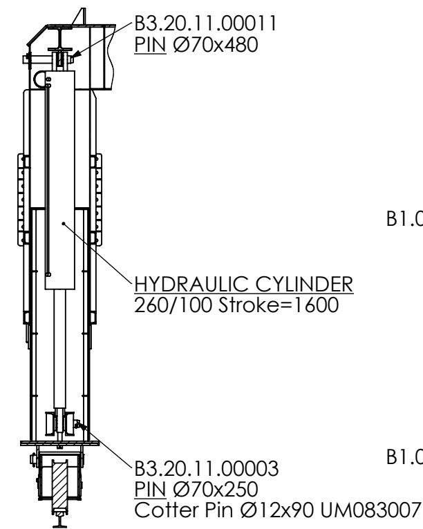
SECTION B-B
