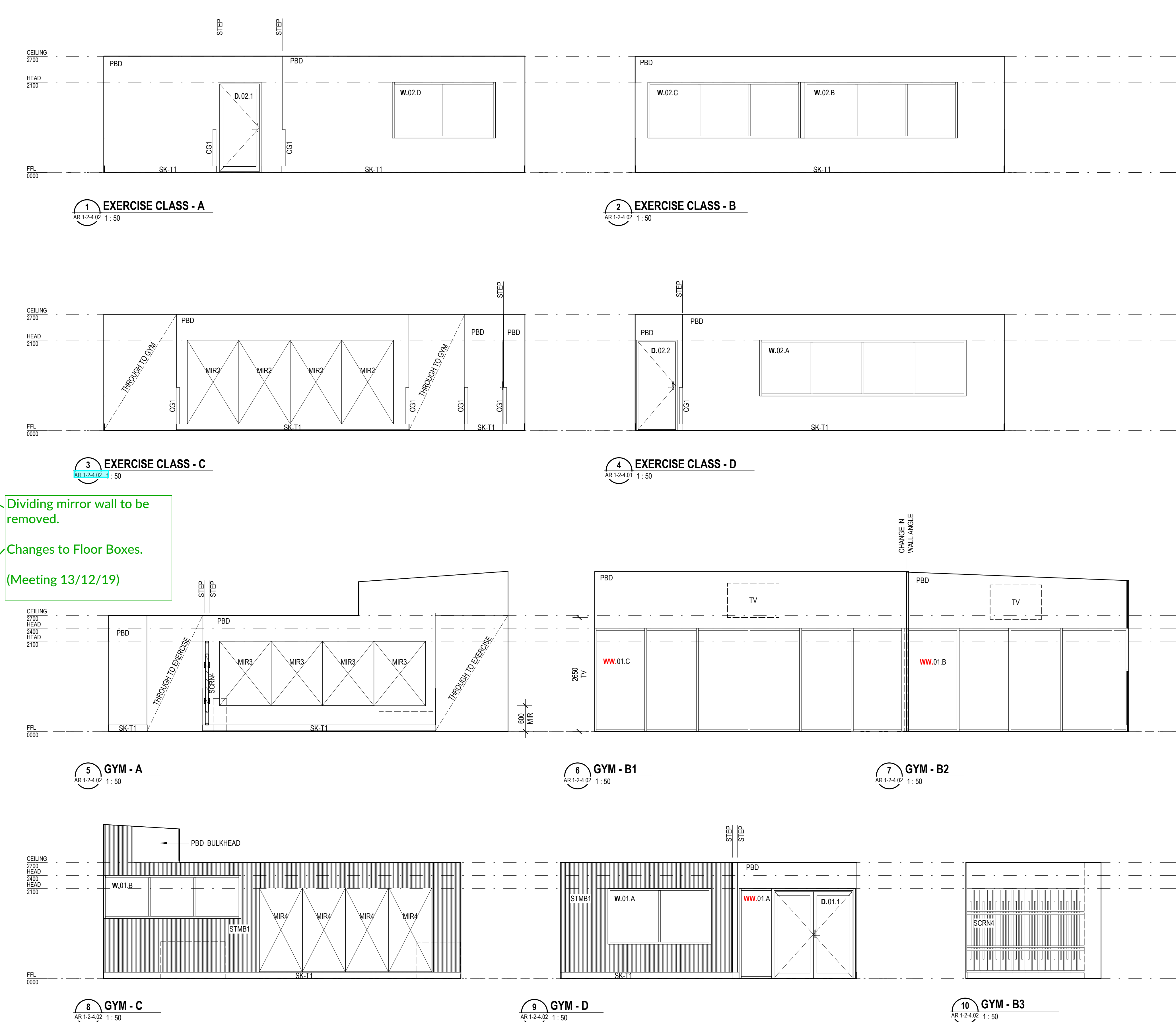
1 EXERCISE CLASS - A AR 1-2-4.02 1 : 50
