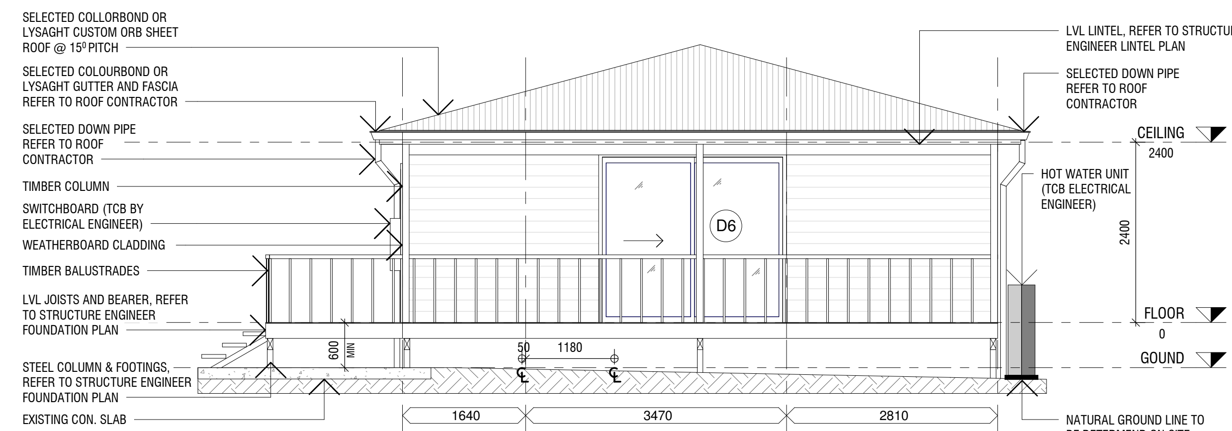
2 NORTHERN VIEW 1 : 50
