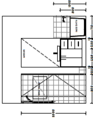
BATH ELEVATION 2
