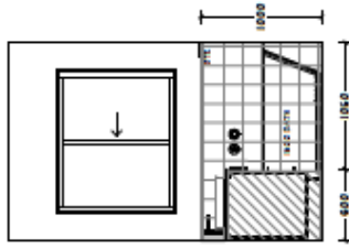
BATH ELEVATION 3
