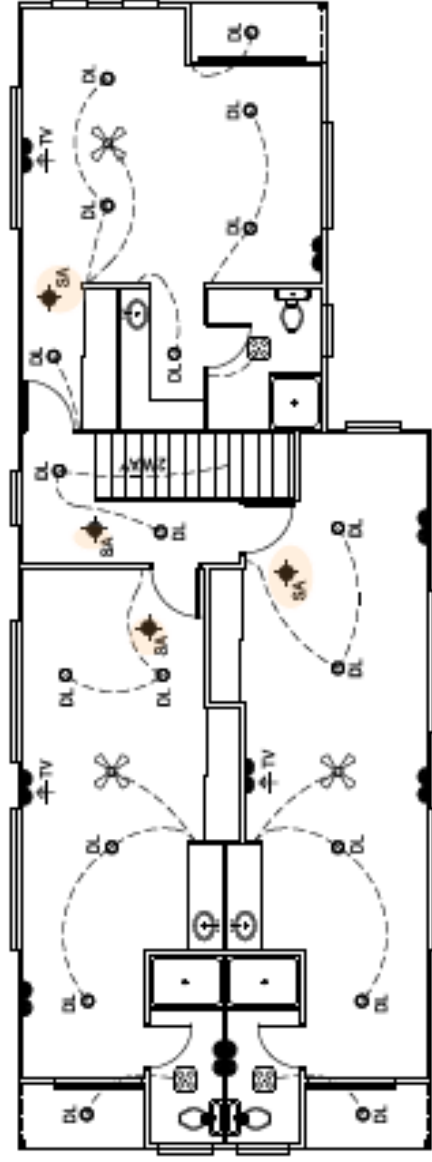
UPPER FLOOR
