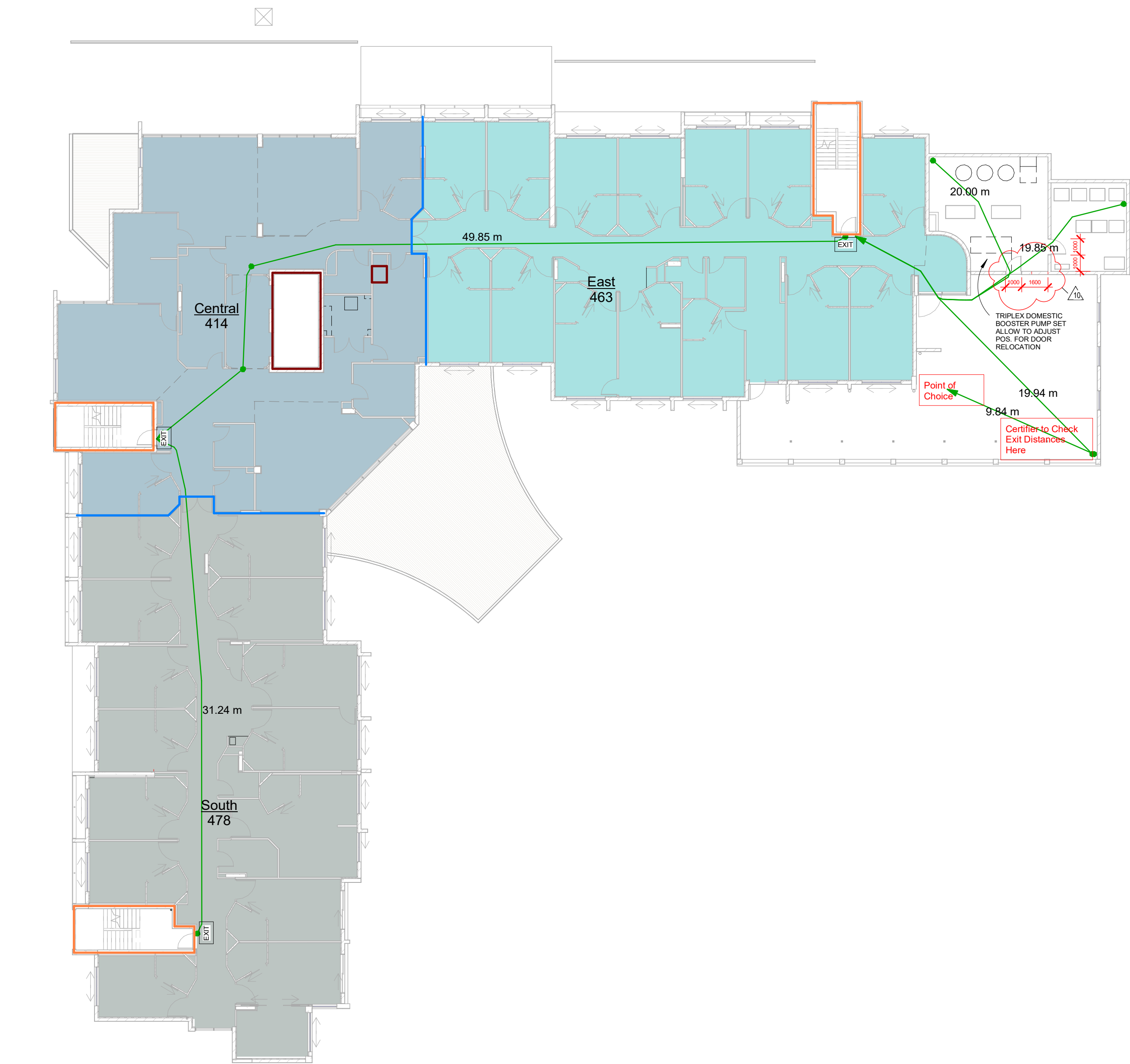
1 Compartmentation - L1 1 : 200
