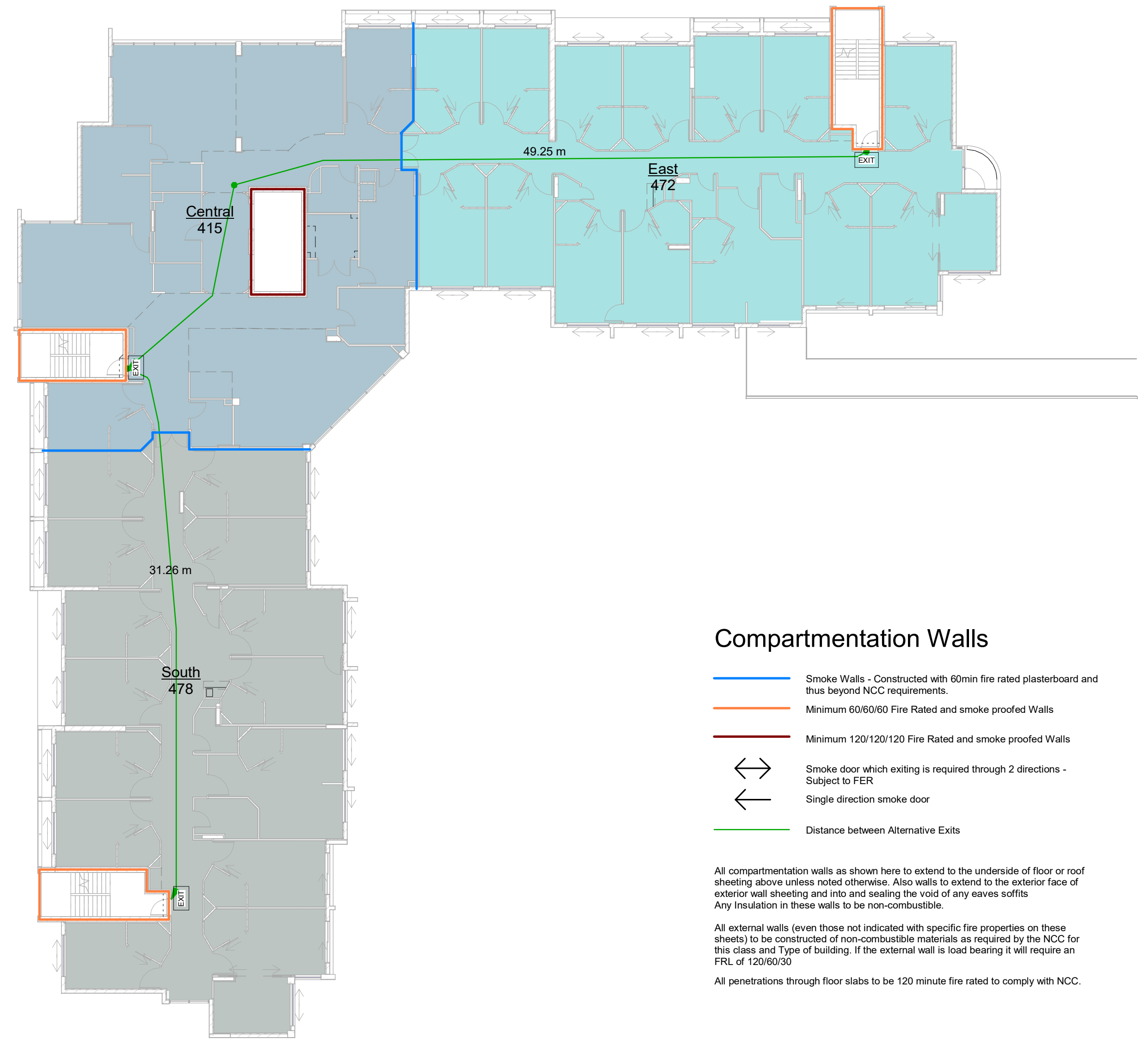
2 Compartmentation - L2 1 : 200
