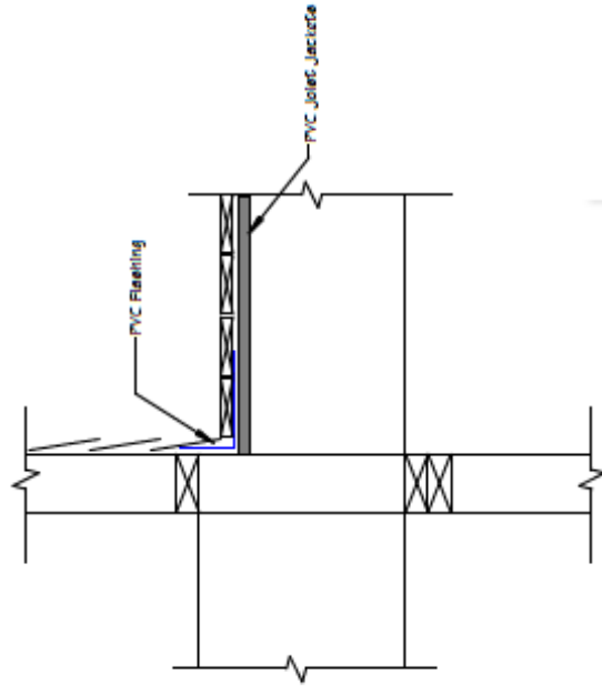
Detail - Timber Deck
