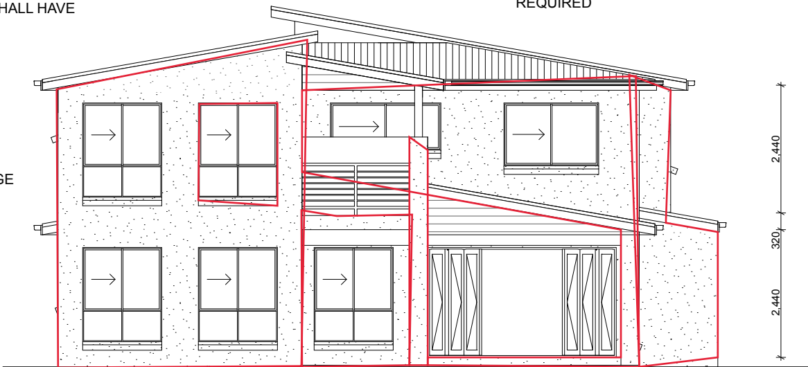
REAR ELEVATION
